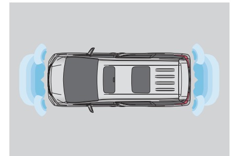
Intelligent Clearance Sonar Eight ultrasonic sensors located in the front and rear side to identify vehicles and all static objects nearby that could cause a potential collision. (All Type)
